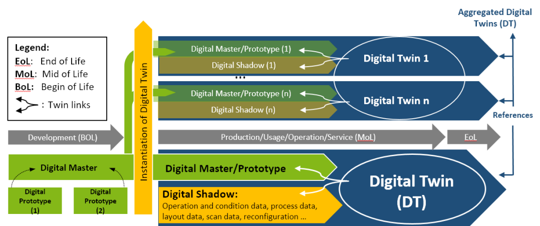
Figure 1: Definition of a digital twin in relation to a product (lower area) and a product instance (upper area) as well as to the digital master, digital prototype and digital shadow
