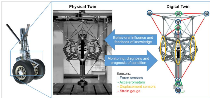
Figure 3: Demonstrator for experimental behavior analysis of an aircraft landing gear with sensor technology for coupling to the digital twin [14, 15]
